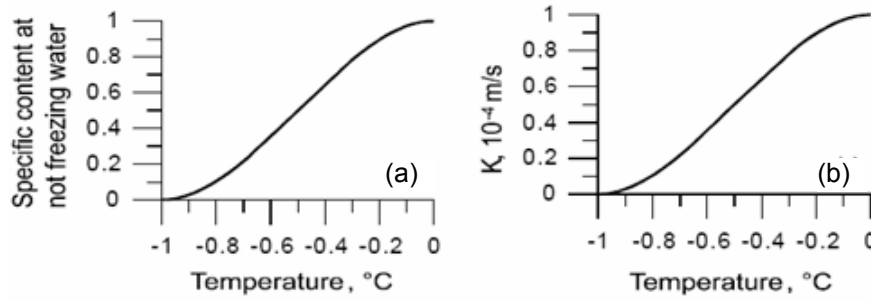
Fig. 2 Variation of the specific contents of non-frozen water (a) and coefficient of permeability K , 10^{-4} m/s (b) as a function of temperature in a zone of phase transfer ( -1^\circ\text{C} up to 0^\circ\text{C} ).
