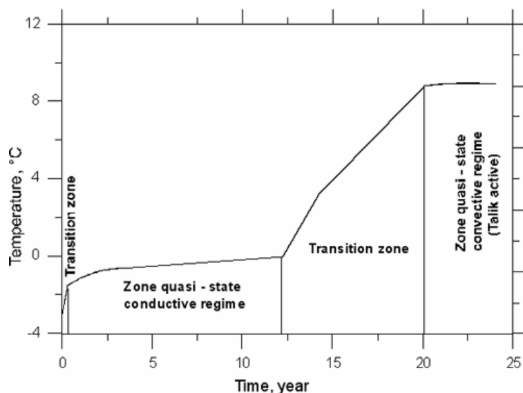
Fig. 3 Variation of seasonal T-maximum at the reference-point situated in the middle of the top of the permeable zone (talik zone) with time. (A–D length on Fig. 1 was 50 m).
